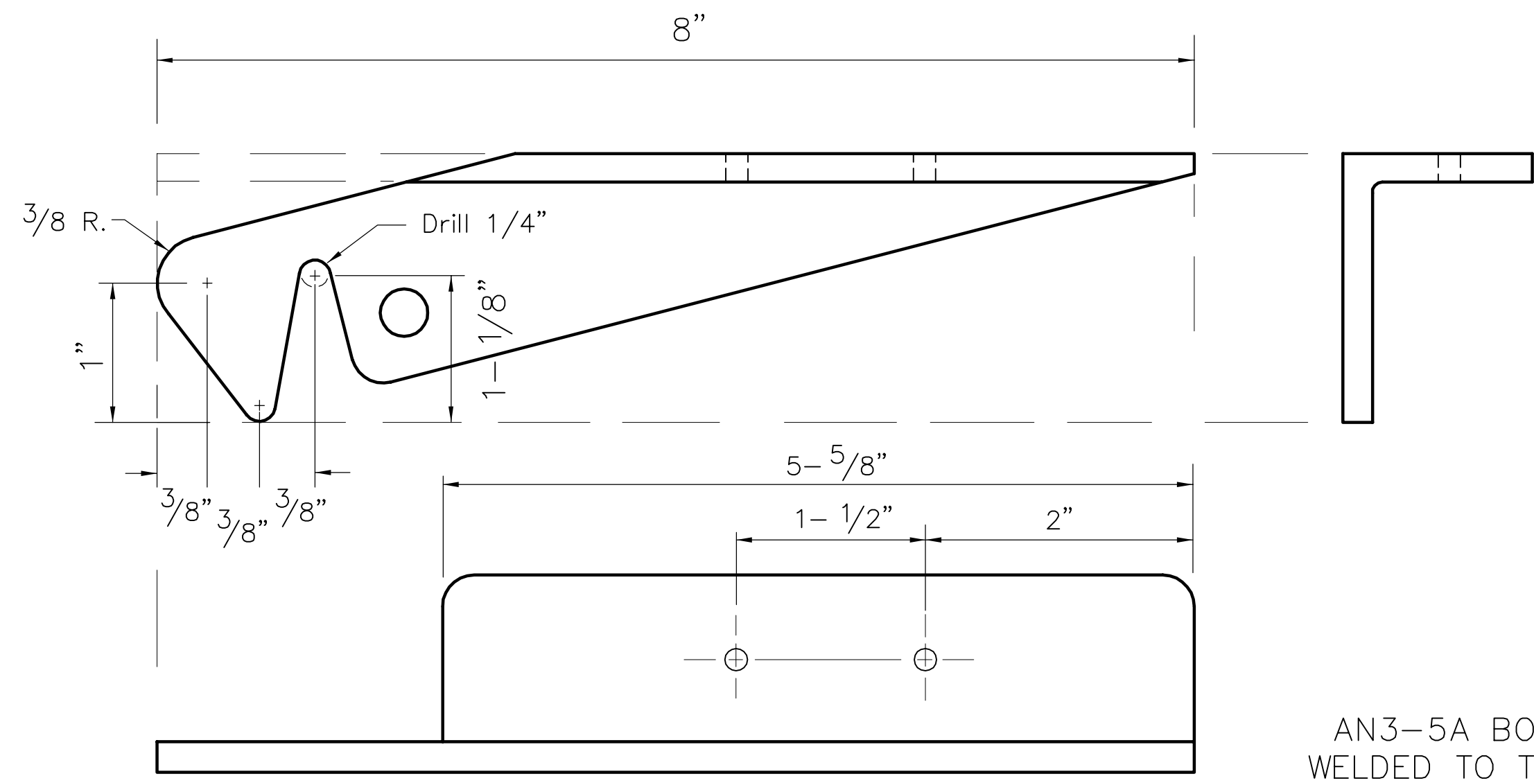
1-1/2" x 2" x 3/16" 6061-T6 ALUM. REQ. 1 LT. / 1 RT. FULL SCALE
